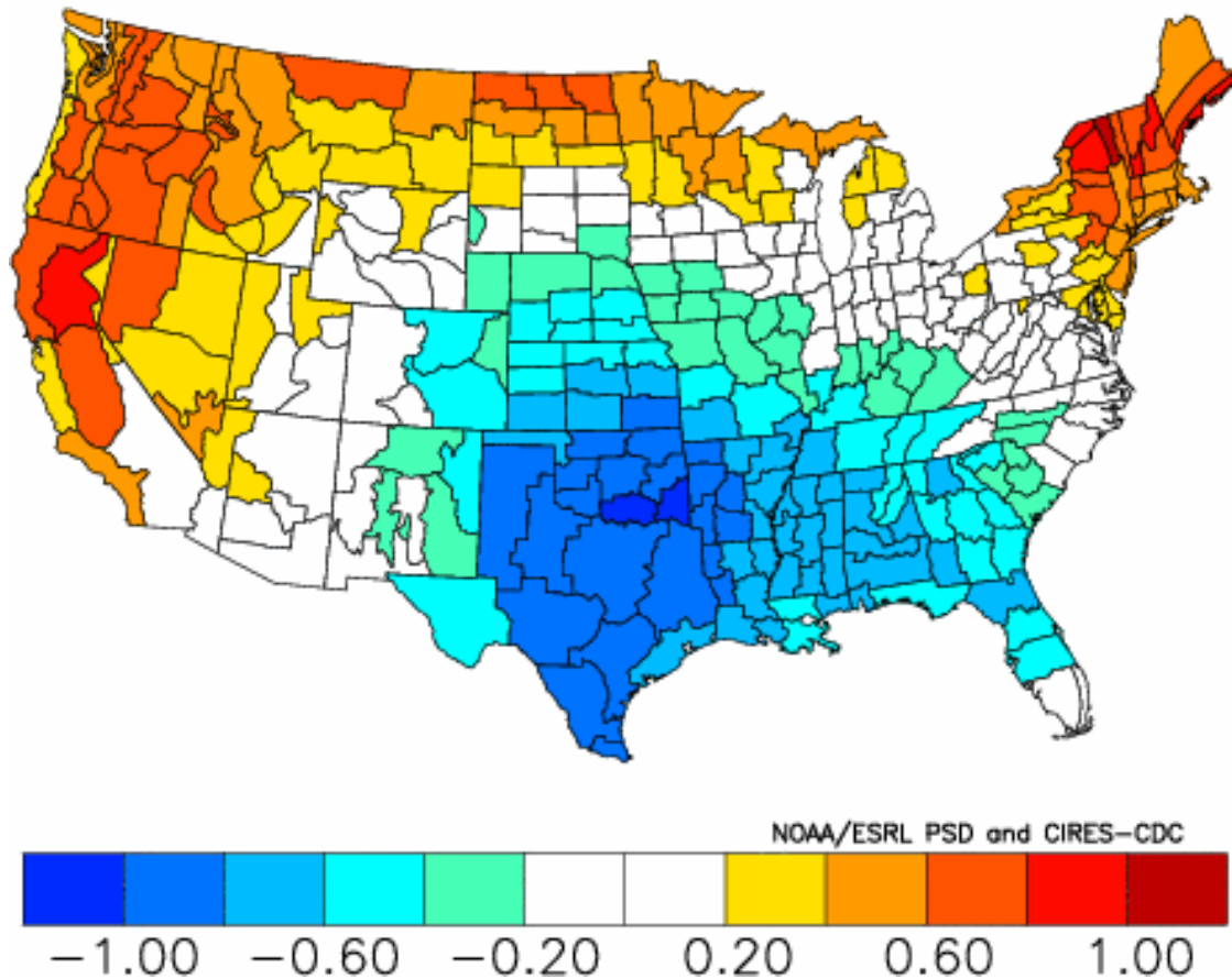
Composite Standardized Temperature Anomalies Aug to Sep 1906,1920,1945,1960,1961,1967,1975,1994,1996,2003 Versus 1895–2000 Longterm Average
